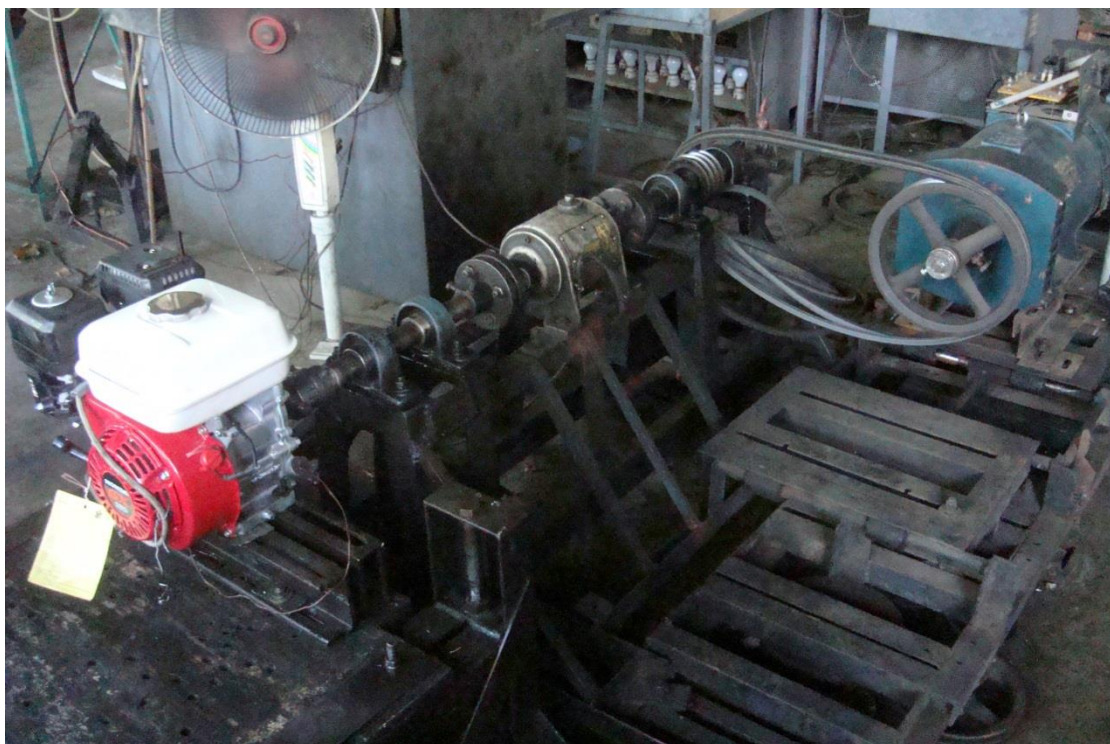
Figure 2. Test set-up of the HONDA GX160 Gasoline Engine
