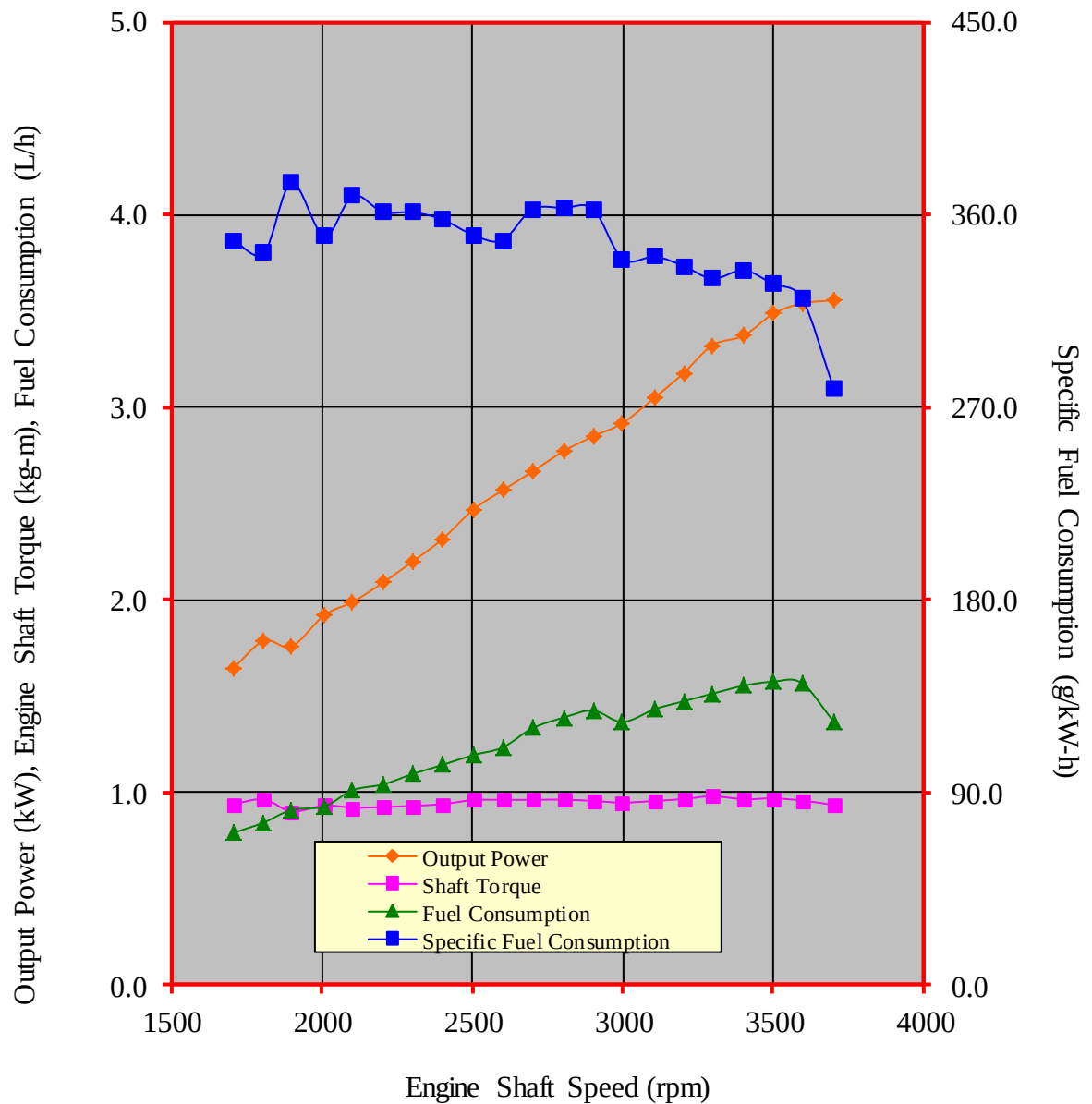
Figure 3. Performance characteristic curves of the HONDA GX160 gasoline engine
