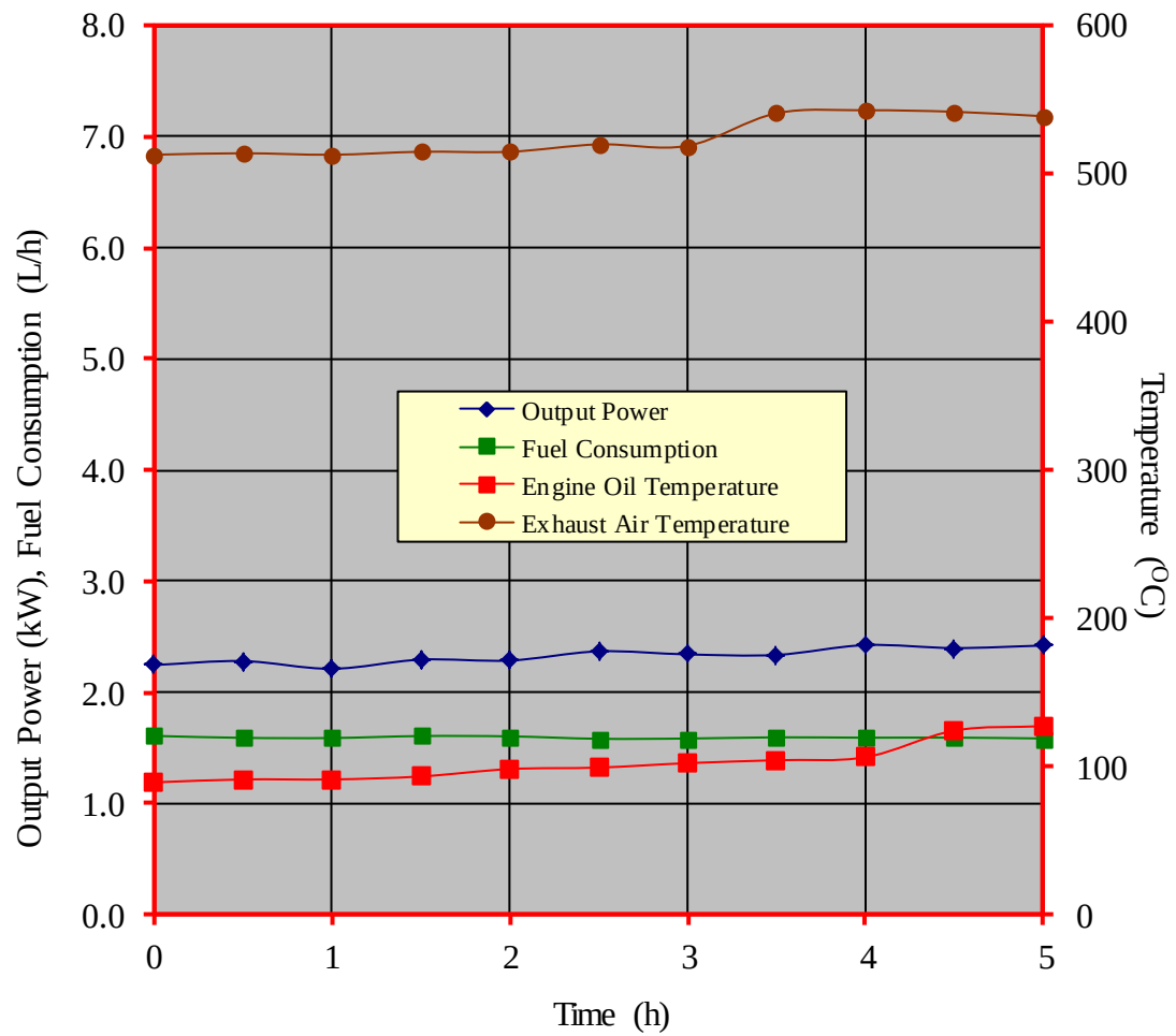
Figure 4. Performance characteristic curves during the continuous running test HONDA GX160 gasoline engine
